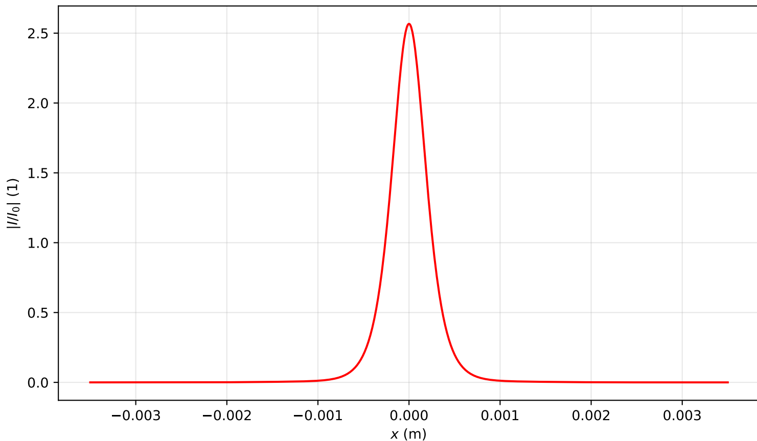
Intensity profile I(x, y = 0, z = 2.866)/I_0 , \text{Pin}=1.0\text{Pcr} , artificial time
